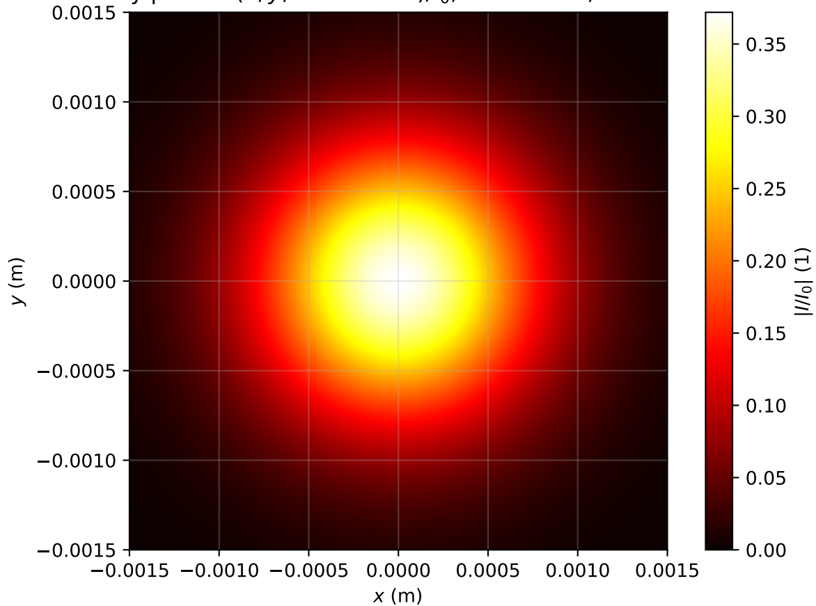
Intensity profile I(x, y, z = 3.662m)/I_0 , P_{in}=0.4P_{cr} , artificial time
